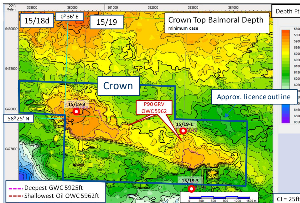
Top Balmoral Depth Map
