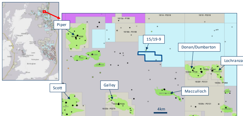
P2366 licence location and neighbouring gas-fields
